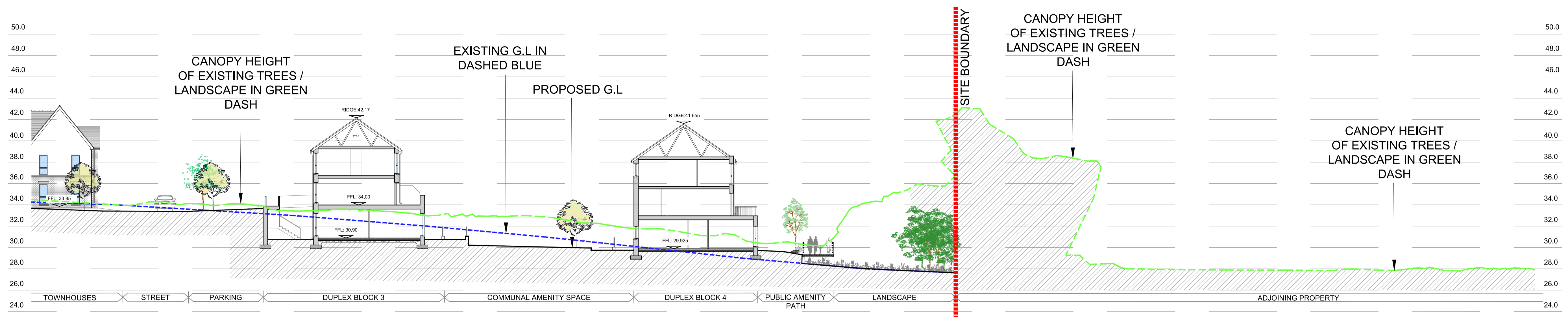
PROPOSED WIDER CONTEXTUAL SECTION P-P 1: 200 @ A1
