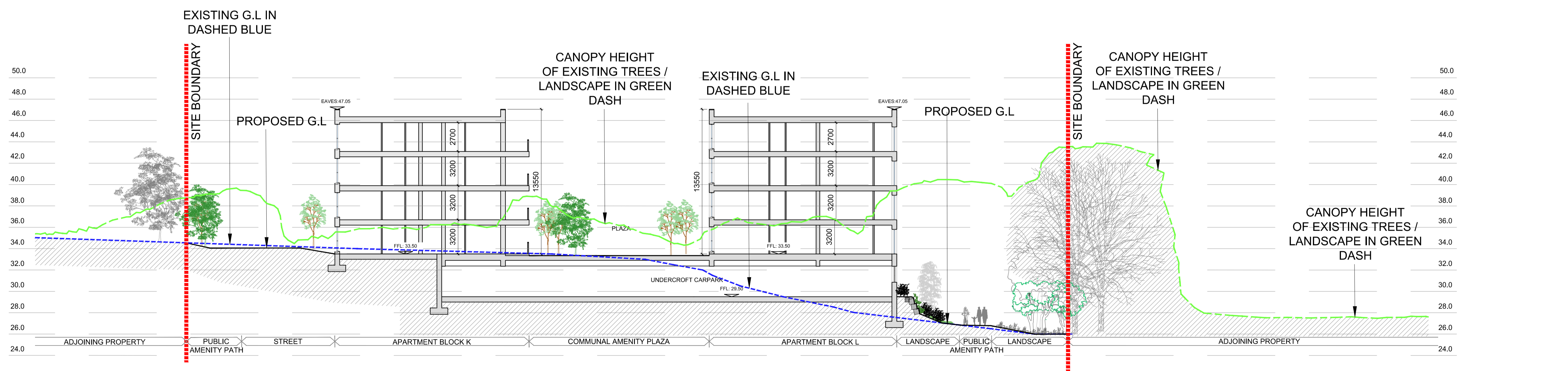
PROPOSED WIDER CONTEXTUAL SECTION Q-Q 1: 200 @ A1
